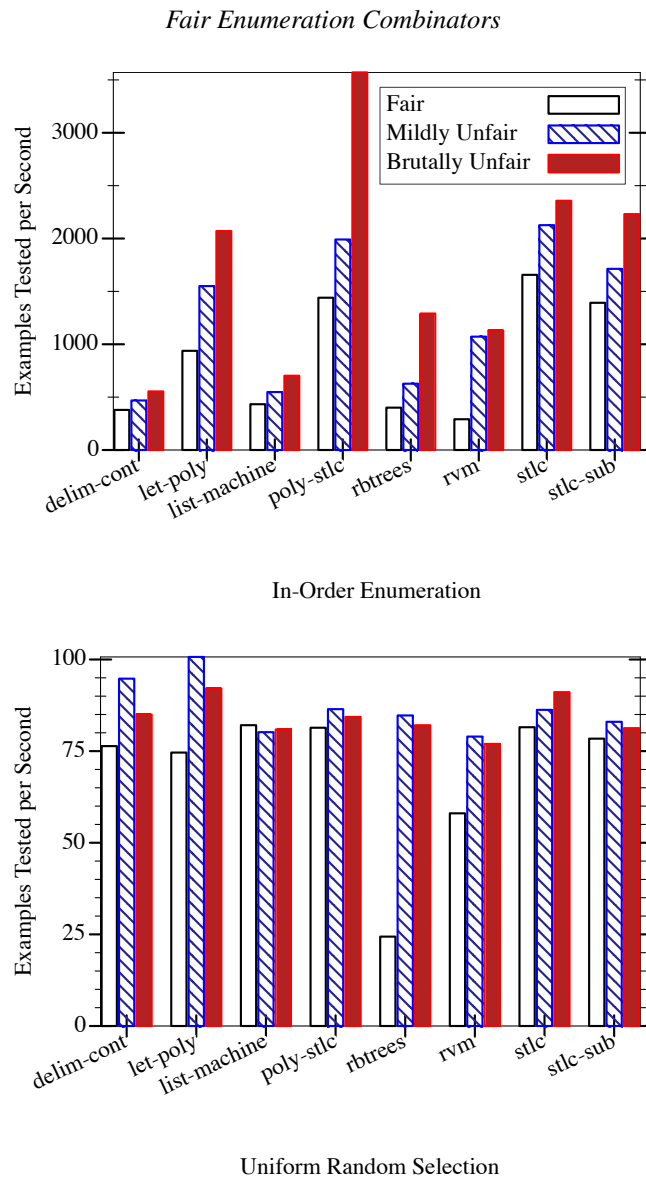
Figure 10: Examples tested per second for each benchmark model and enumeration-based generator
